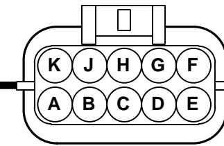
View: Wire Insertion Side
